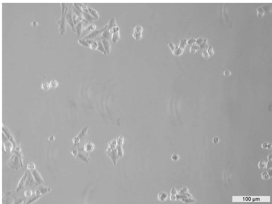
15042909 CHO-K1.CI-0236/CHO-K1.CI-0239 Early log phase
