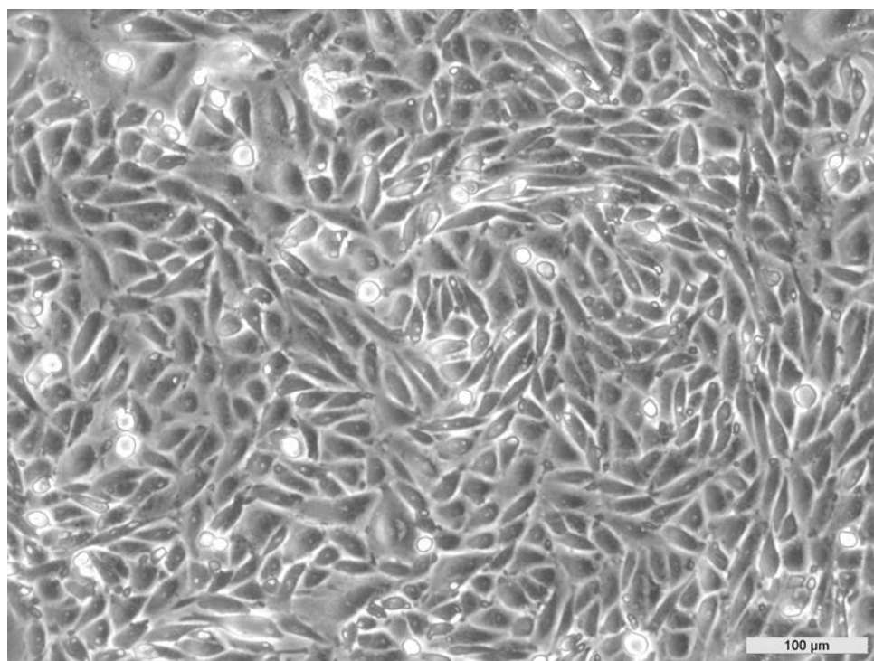
15042909 CHO-K1.CI-0236/CHO-K1.CI-0239 late log phase
